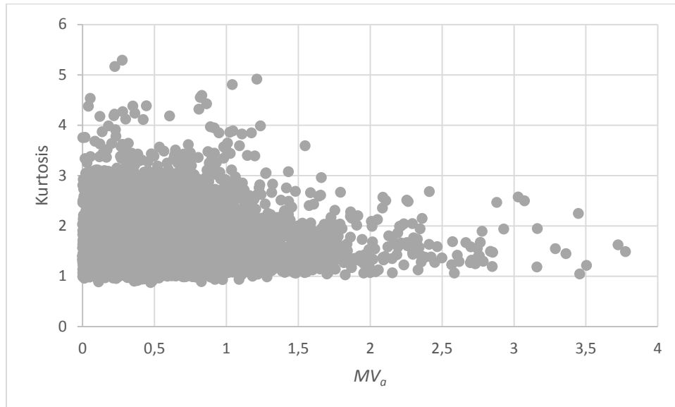
FIGURE 6. SIMULATION 3: KURTOSIS VS MV_a (AFTER 350 TIME PERIODS)
