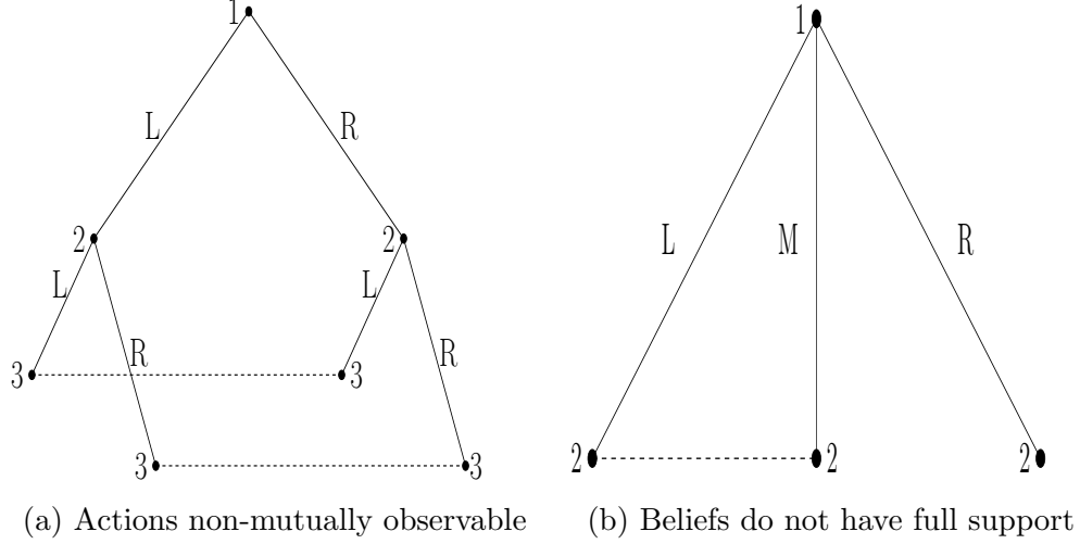
Figure 4: Continuous beliefs not possible
