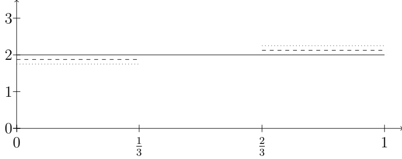
Figure 1: Belief entanglement
