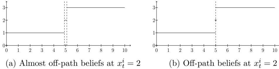
Figure 5: Continuity of beliefs
