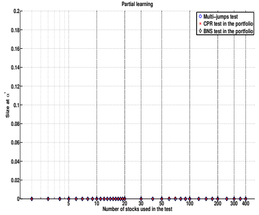
Figure 13: Shows the power and size (at 5% and \alpha^* confidence levels) of the multi-jump on N stocks and of the CPR and BNS tests on the portfolio of N simulated stocks, as a function of N . The left panels show the result in the case with no partial adjustment. The right panels show the case in which partial adjustment effects are added to the baseline model. Solid lines are for the case in which the N stocks are selected according to the highest learning parameter; dashed lines are for the case in which the stocks are selected randomly.
