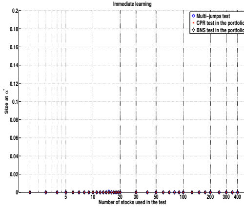
Figure 13: Shows the power and size (at 5% and \alpha^* confidence levels) of the multi-jump on N stocks and of the CPR and BNS tests on the portfolio of N simulated stocks, as a function of N . The left panels show the result in the case with no partial adjustment. The right panels show the case in which partial adjustment effects are added to the baseline model. Solid lines are for the case in which the N stocks are selected according to the highest learning parameter; dashed lines are for the case in which the stocks are selected randomly.
