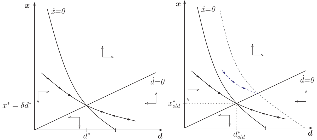
Left panel: Phase diagram with stable saddlepath. Right panel: Phase diagram used for proof of Lemma 1.
