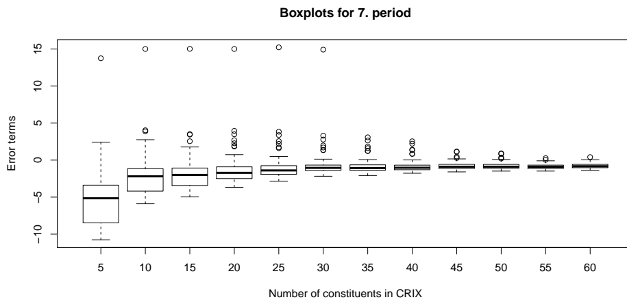
Figure 7: Boxplots for the last 3 periods of CRIX error terms
