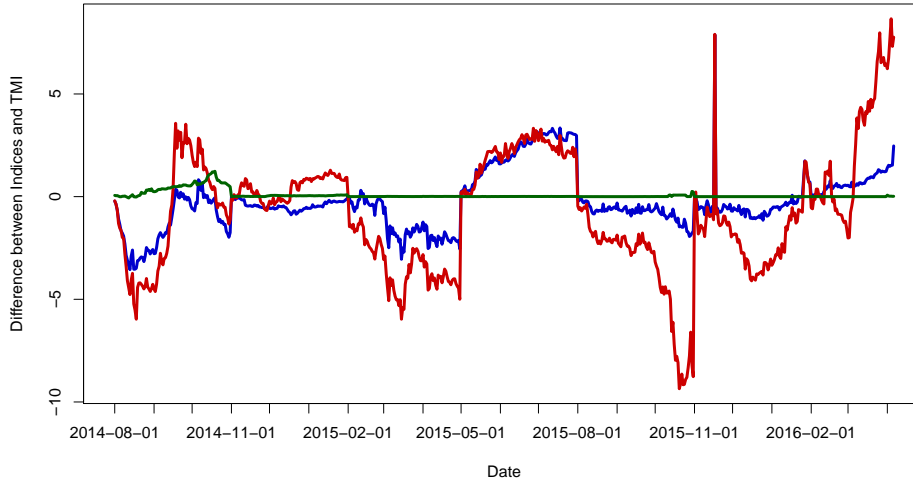
Figure 2: Realized difference between TMI and CRIX , ECRIX , EFCRIX CRIXfamdiff CRIXcode
