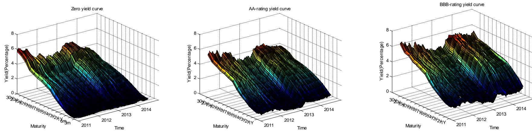
Fig. 1. Time series plot of Treasury zero, AA- and BBB-rated yield curves The sample consists of daily Treasury zero, AA- and BBB-rated yield data across various maturities from Jan. 2011 to Dec. 2014.
