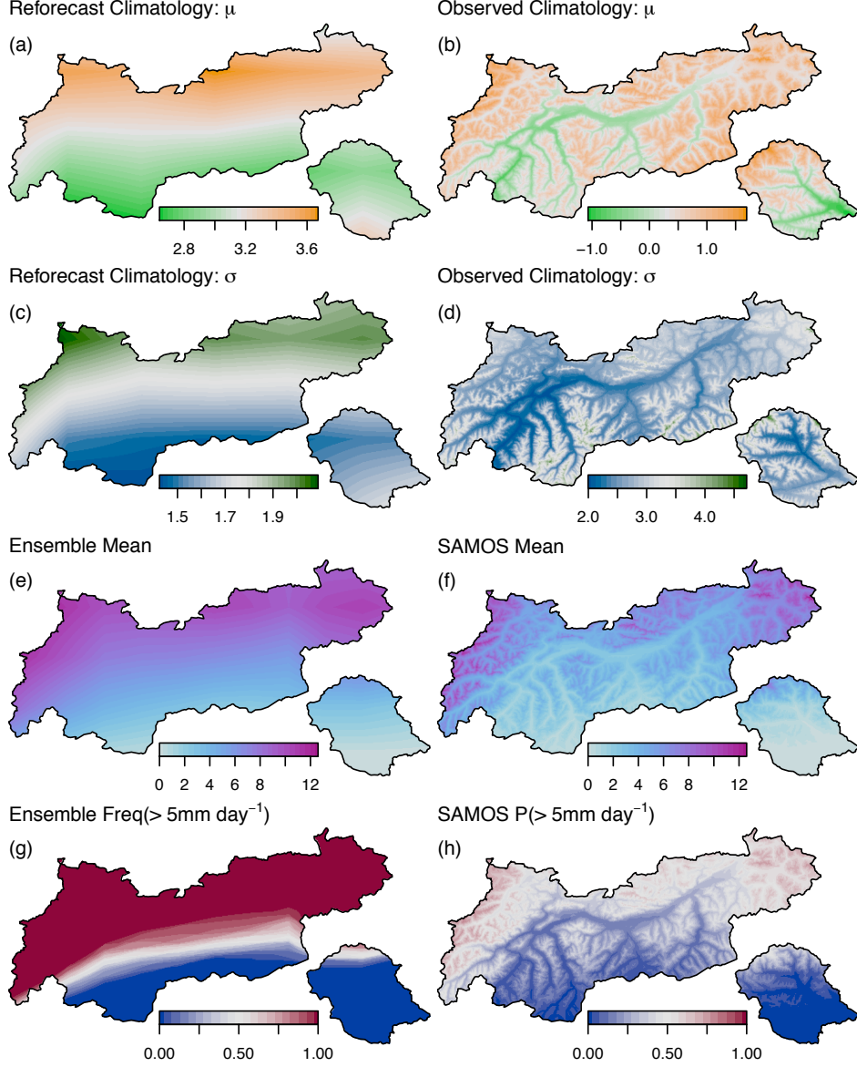
Figure 3: Example prediction for May 18, 2010, one-day-ahead forecast. Left column shows reforecast climatologies and the raw ensemble forecast; right column shows the observed climatology, and the post-processed SAMOS predictions. Top down: climatological location ( \mu ; (a), (b)), climatological scale ( \sigma ; (c), (d)), forecast mean ((e), (f)), and frequency (g) and probability (h) of exceeding 5 \text{ mm day}^{-1} . Location \mu and scale \sigma on the latent power-transformed scale in \text{mm}^{\frac{1}{p}} with p = 1.35 . Note that (a)/(b) and (c)/(d) use different color scales regarding the range of the data.
