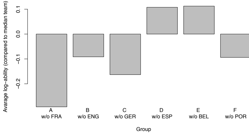
Figure 4: Group strengths. Average log-ability within each group, excluding the group favorite and centered by median log-ability across all teams.
