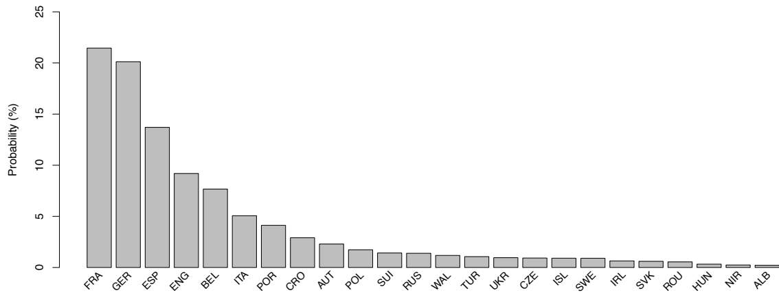
Figure 1: Euro 2016 winning probabilities from the bookmaker consensus model.
