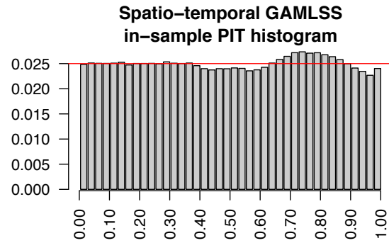
Figure 11: Pit histogram of the spatio-temporal GAMLSS model evaluated on the training data set. Width of the bins: 2.5%.
