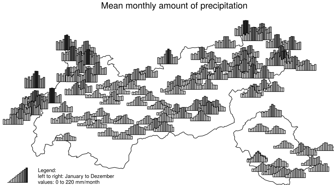
Figure 3: Mean monthly precipitation in millimetres, based on the data set. Each bar indicates one month (January–December, left to right). Bar height and luminance contain the same information.
