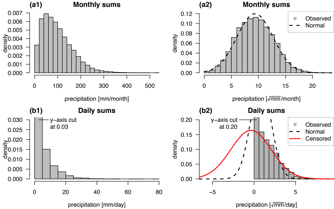
Figure 1: Density plot of precipitation sums. Top row: monthly precipitation sums from 117 stations. Bottom row: daily precipitation sums of one sample station. Right column: power-transformed observations ( \sqrt{\text{mm}} \text{ day}^{-1} ) with a normal distribution fitted to it (black, dashed). Additionally a left-censored normal distribution is fitted to the power-transformed daily observations (bottom right; red, solid). Please note: y-axes in the bottom row are both cut.
