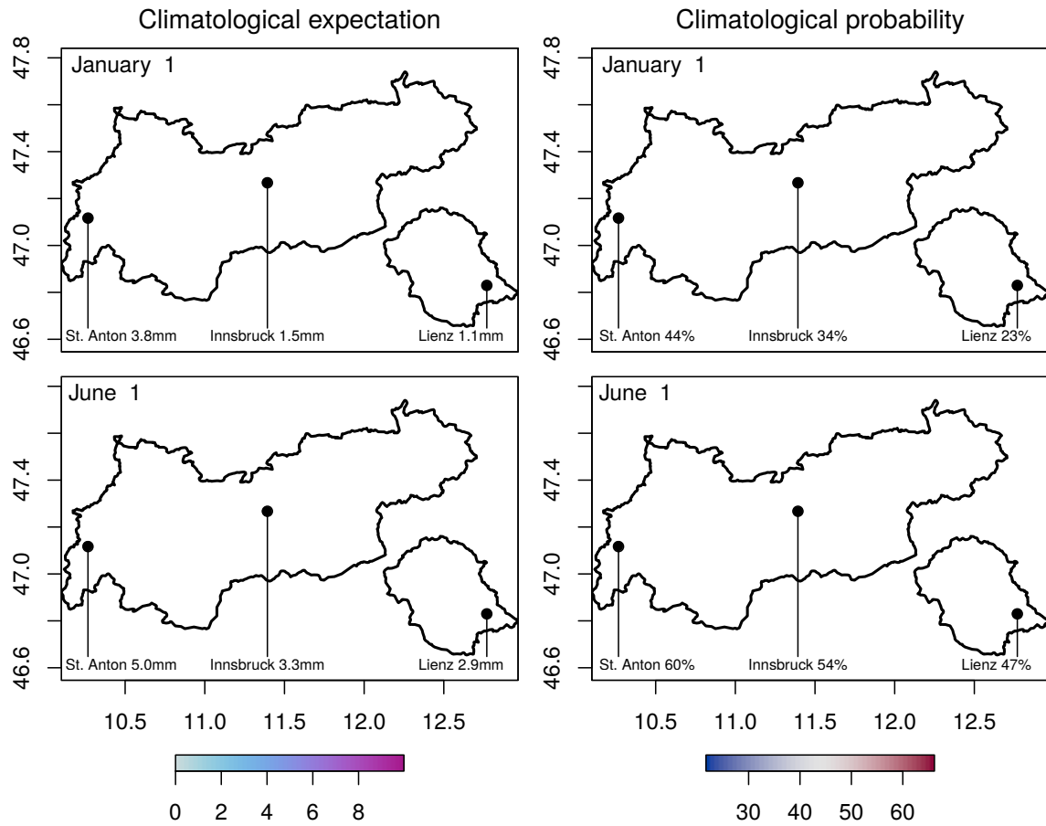
Figure 9: Climatological expectation (left; \text{mm day}^{-1} ), and climatological probability of precipitation (right; %) for January 1 (top panel), and June 1 (bottom panel) respectively. Values explicitly shown for three locations: St. Anton (1284 m amsl ), Innsbruck (574 m amsl ), and Lienz (673 m amsl ). Prediction based on the SRTM digital elevation model (CGIAR-CSI 2016).
