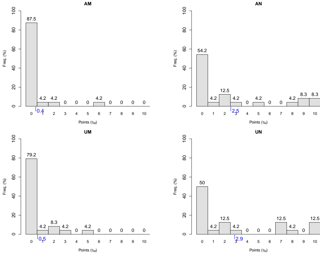
Figure 3: Punishment
