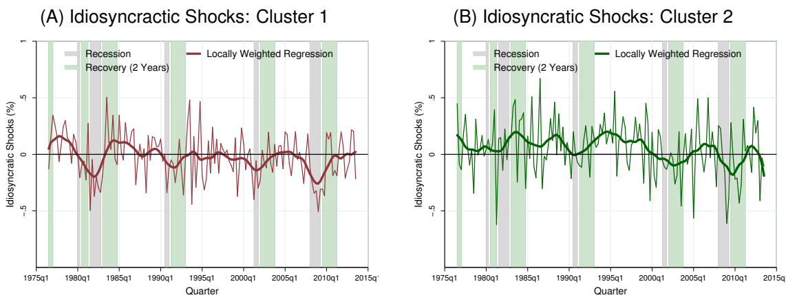
Figure 6: Idiosyncratic Dynamics
