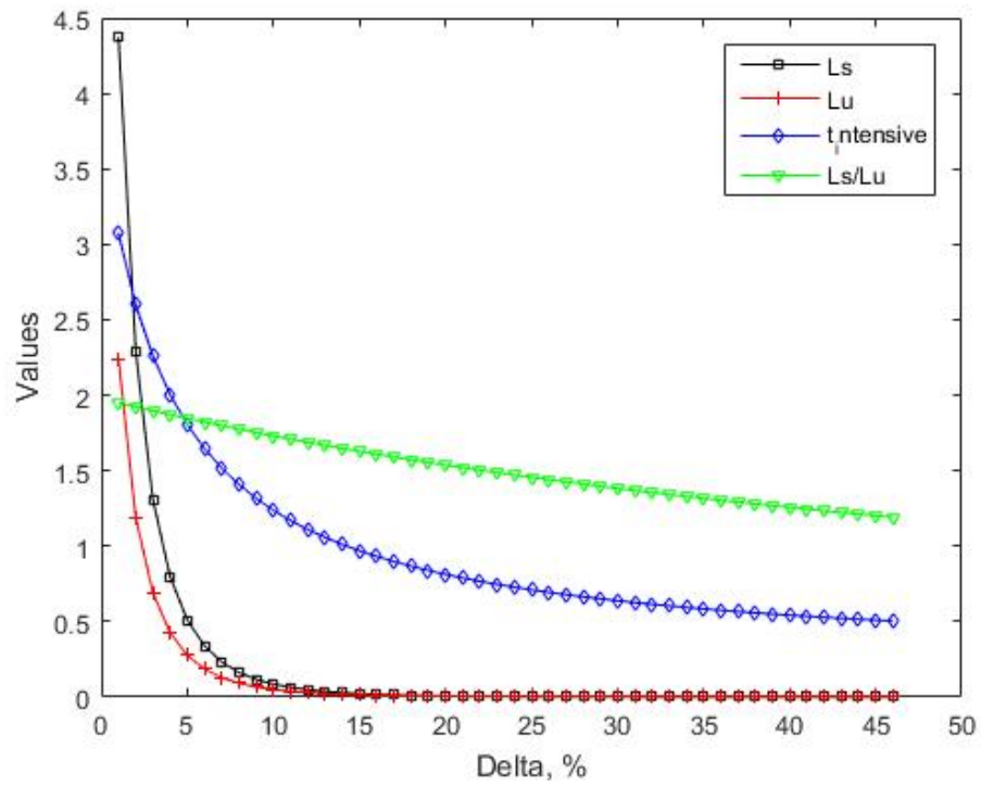
Figure 1: Results from the simulation of our theoretical framework I
