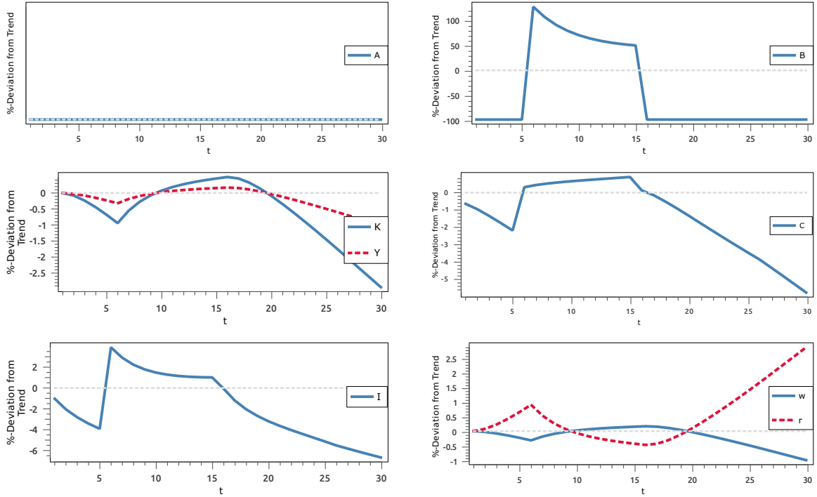
Figure 2: Bubble-driven business cycles
