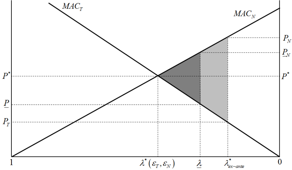
Figure 1: Abatement costs of partitioned environmental regulation under “first-best” [\lambda^*(\epsilon_T, \epsilon_N), P^*(\epsilon_T, \epsilon_N)] , “second-best” pure quantity-based [\lambda_{ex-ante}^*] and hybrid [\underline{\lambda}] policies
