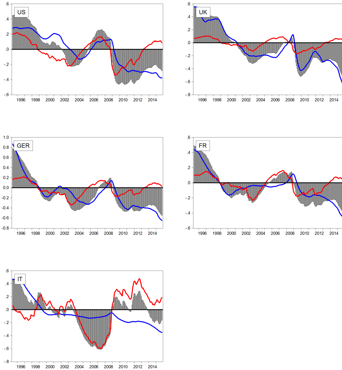
Figure 4: Country-wise monthly long-term correlation component (gray area) and its contributions from the monetary policy factor ( m_{MP} , blue line) and from realized volatility ( m_{RV} , red line) from the bivariate DCC-MIDAS-X model estimations in Table 8.
