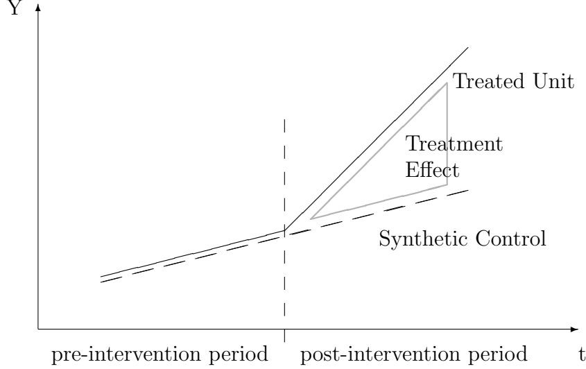
Figure 1: Stylised Representation of the Synthetic Control Method
