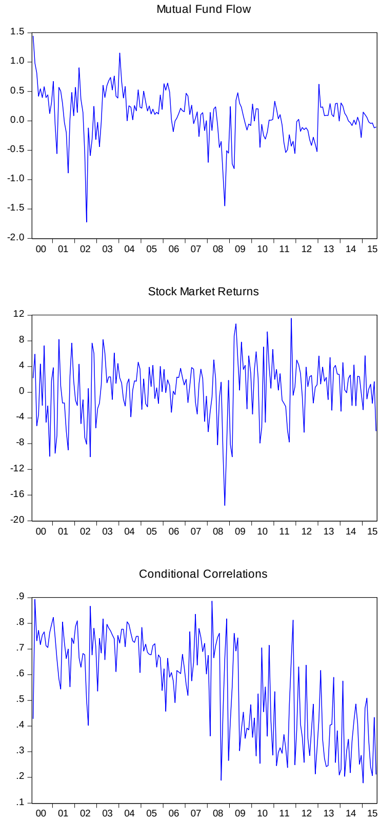
Figure 1: Mutual Fund Flow, Stock Market Returns and Conditional Correlations
