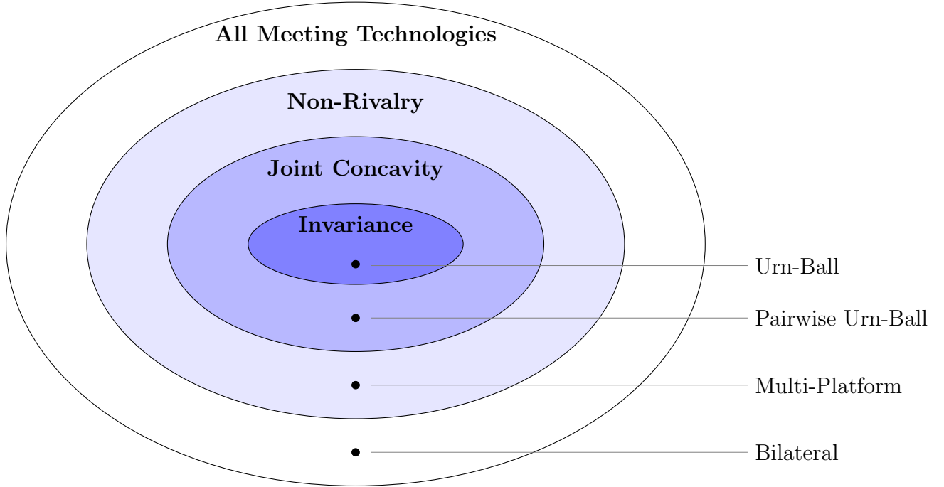
Figure 1: Venn Diagram of Meeting Technologies
