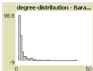
Figure A1: Artificial network – „Erdős-Rényi“ vs. „Barabasi-Albert“ model Source: Simulation model applied in: Müller et al. (2015)
