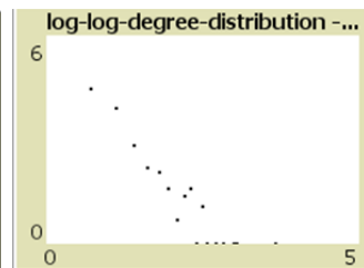
Figure A1: Artificial network – „Erdős-Rényi“ vs. „Barabasi-Albert“ model Source: Simulation model applied in: Müller et al. (2015)
