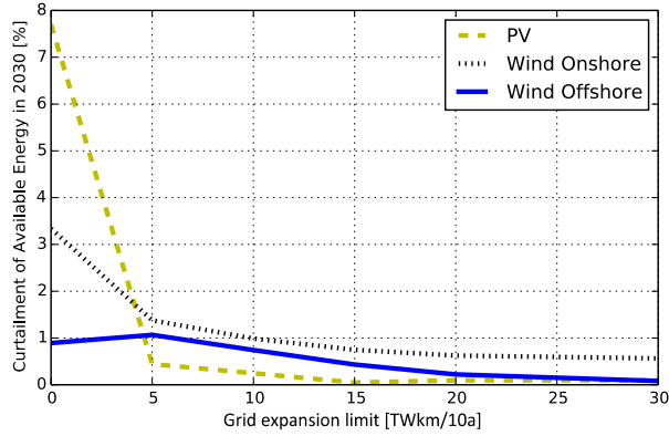
Figure 7: Curtailment of renewables for the different scenarios
