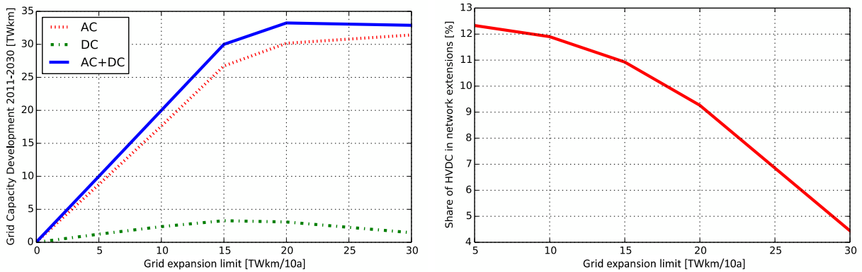
Figure 10: Total capacity development for 2011-2030 (left) and the share of DC in the total network expansion (right)
