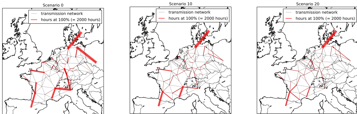
Figure 5: Line load after redispatch measures in different scenarios 2020
