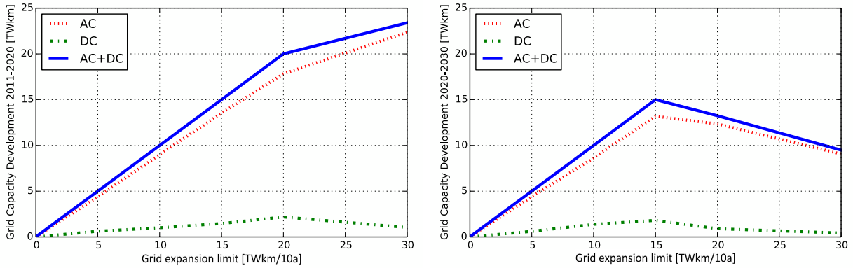
Figure 9: Capacity development in TWkm for the period 2011-2020 (left) and 2020-2030 (right)
