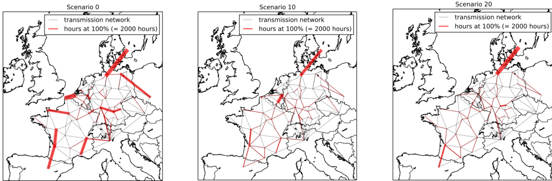
Figure 6: Line load after redispatch measures in different scenarios 2030
