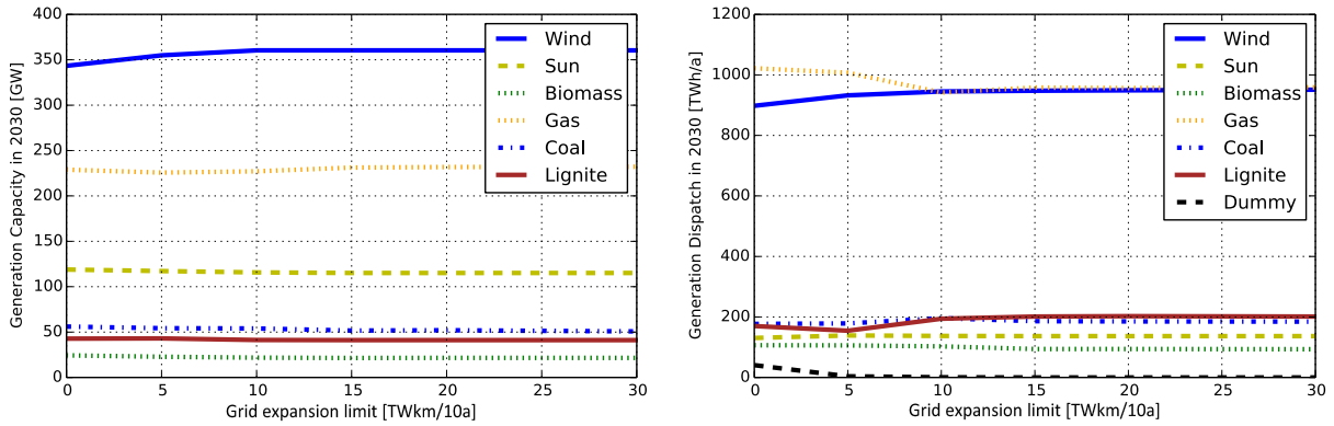
Figure 12: Total generation capacity (left) and yearly dispatch (right) in 2030 for the different grid restriction scenarios
