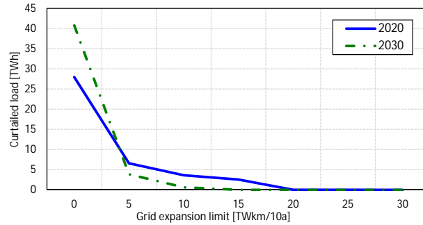
Figure 2: Curtailed load in different scenarios
