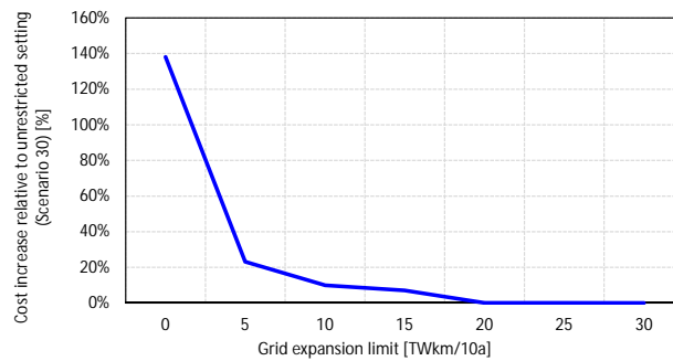
Figure 8: Total system cost decrease with grid expansion
