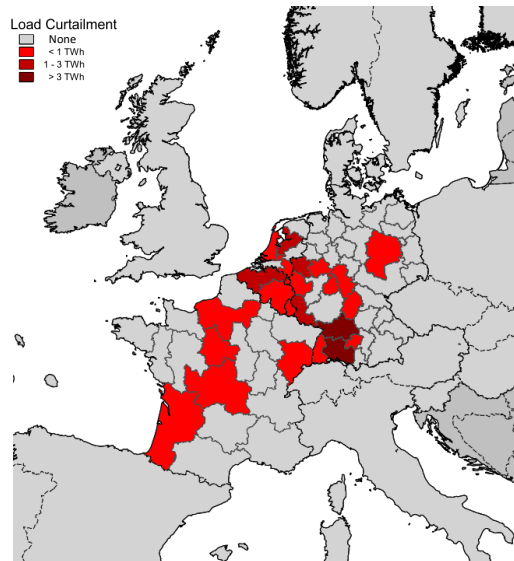
Figure 3: Geographical distribution of load curtailment in Scenario 0 for 2030
