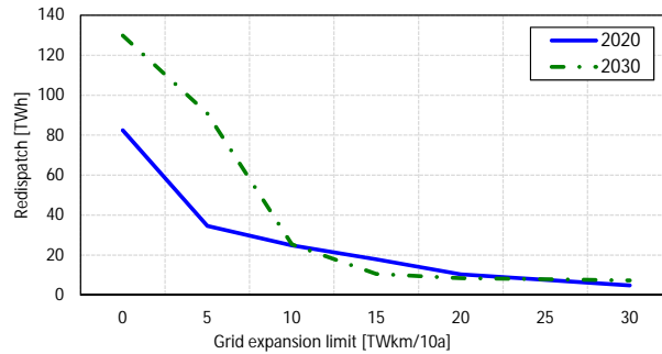
Figure 4: Redispatch measures in different scenarios
