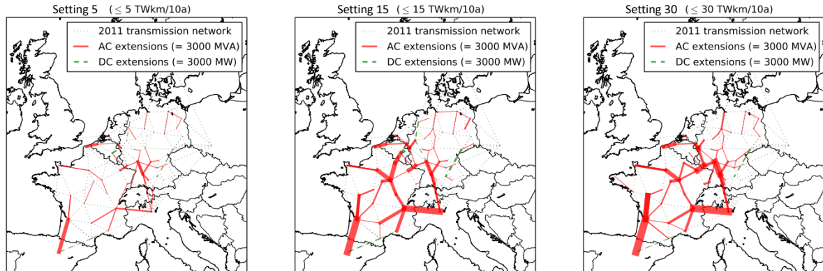
Figure 11: Maps of grid expansion for scenarios 5, 10 and 30
