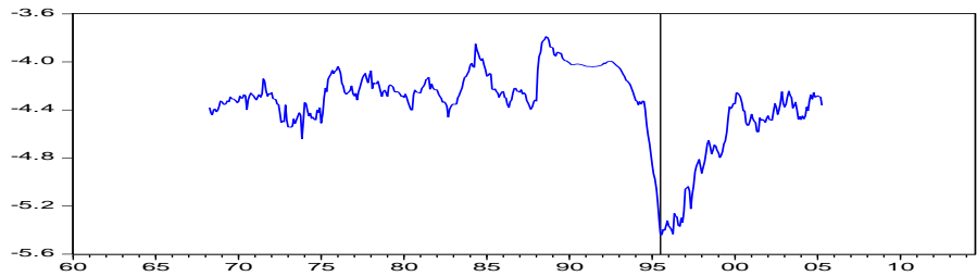
Figure 2: Zivot-Andrews Breakpoint Test
