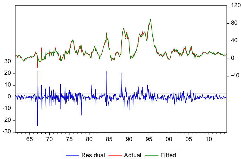
Figure 2: Residual graph
