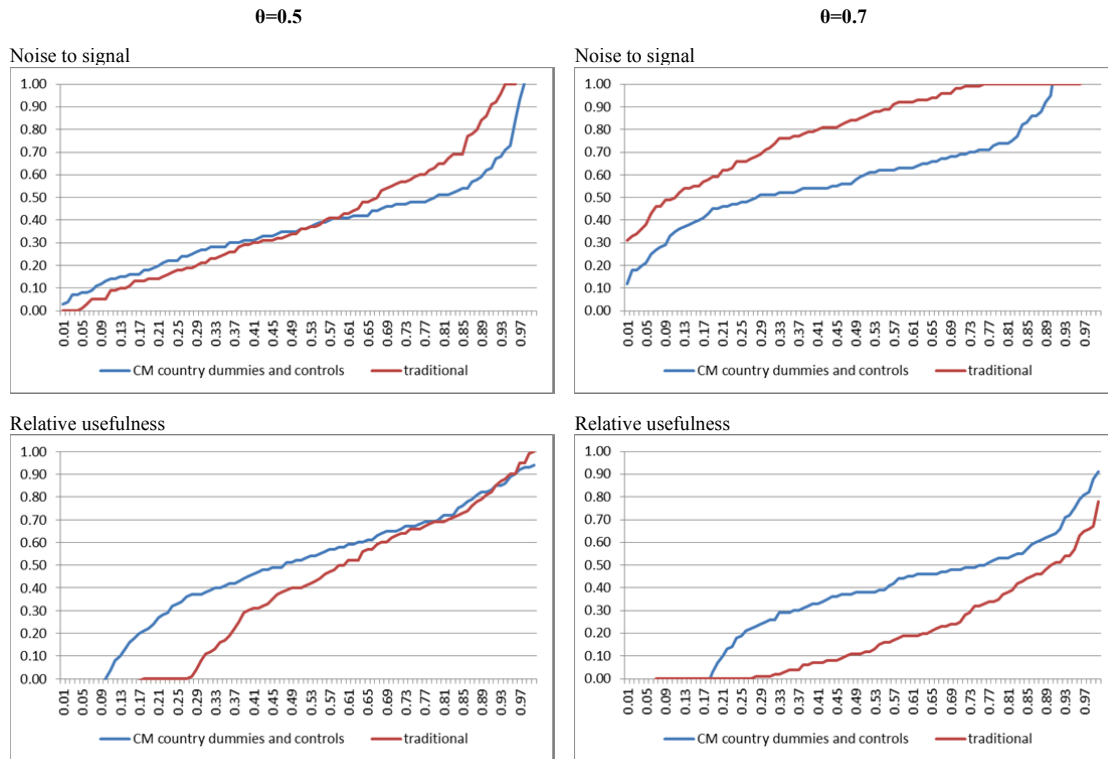
Figure 5: Distribution of noise to signal ratios and relative usefulness across country/indicator pairs
