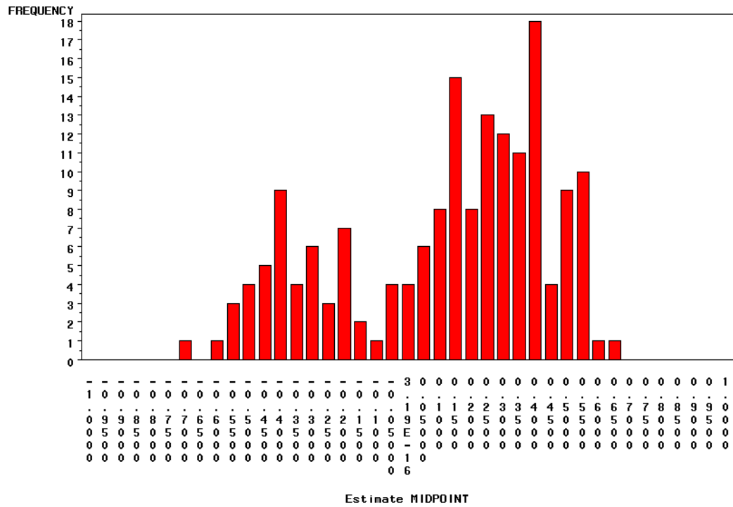
The histogram of the estimates of the gradualism parameter \gamma for the NEIG category.
