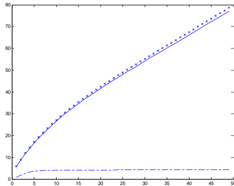
Figure 11(b) \kappa = 3
