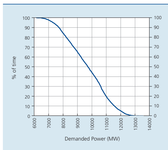
CHART 5 LOAD DURATION CURVE FOR BELGIUM
