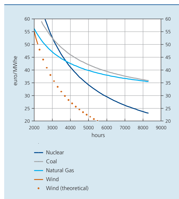
CHART 4 AVERAGE PRODUCTION COSTS OF ELECTRICITY GENERATING STATIONS, INCLUDING CO 2 COSTS (10 €/tCO 2 )
