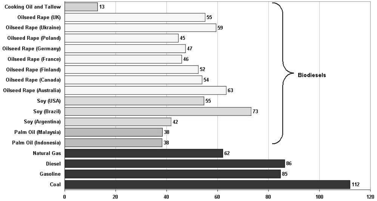
Figure 1: Carbon intensity of biofuels and fossil fuels. Source: UK Government. Notes: X axis measures the CO 2 in gram produced per Megajoule of energy.
