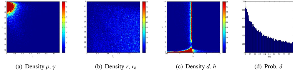
Figure 7: Computed parameter densities for saddle-saddle optimal scenarios
