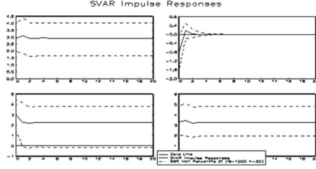
Fig. 1. Responses of "ind" and "rent" (top to bottom) to real shock (left) and nominal shok (right) with 95% Hall percentile bootstrap confidence interval based on 1000 bootstrap replications(ALGERIA).
