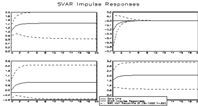
Fig. 2. Responses of "ind" and "rent" (top to bottom) to real shock (left) and nominal shok (right) with 95% Hall percentile bootstrap confidence interval based on 1000 bootstrap replications(CHINA).
