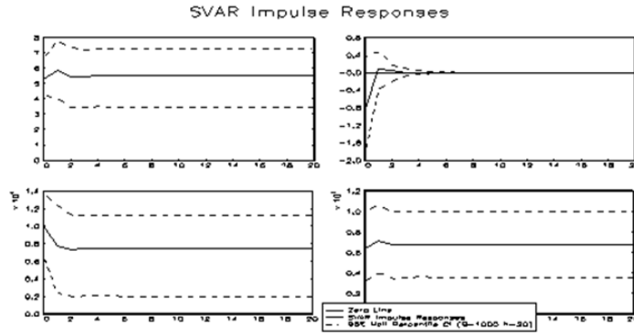
Fig. 6. Responses of "ind" and "rent" (top to bottom) to real shock (left) and nominal shock (right) with 95% Hall percentile bootstrap confidence interval based on 1000 bootstrap replications (SAUDI ARABIA).
