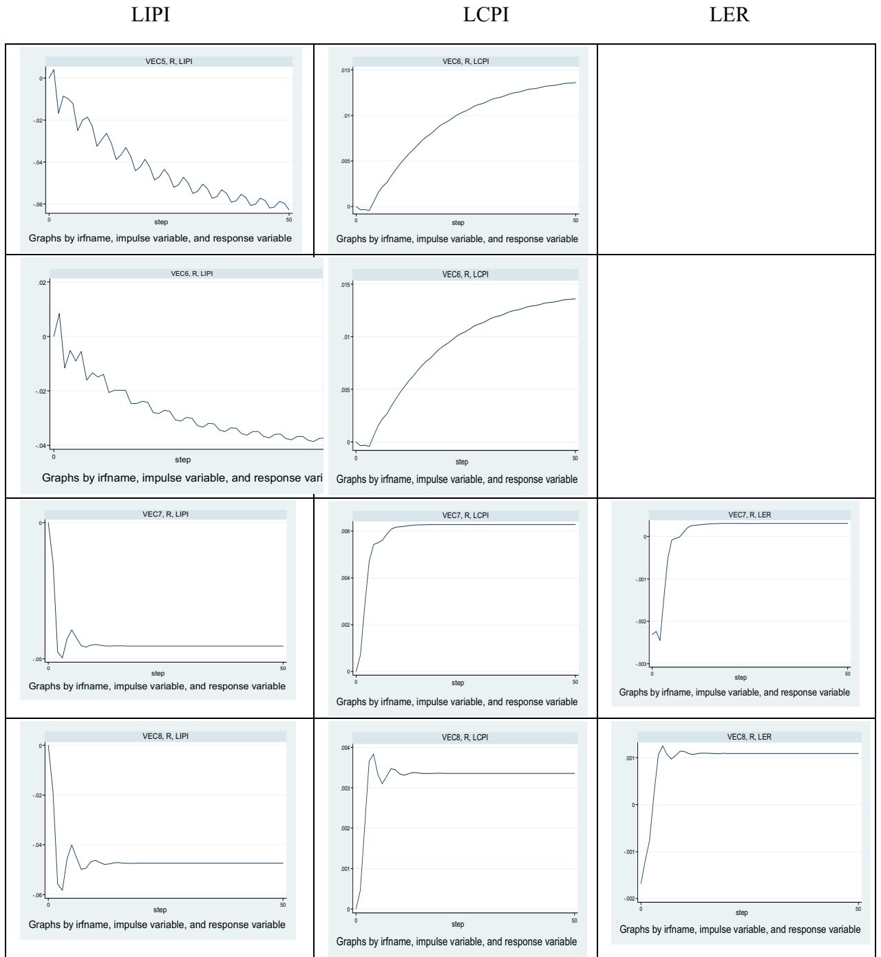
Figure 3: IRFs: Effects of Shocks to Short-term Interest Rate
