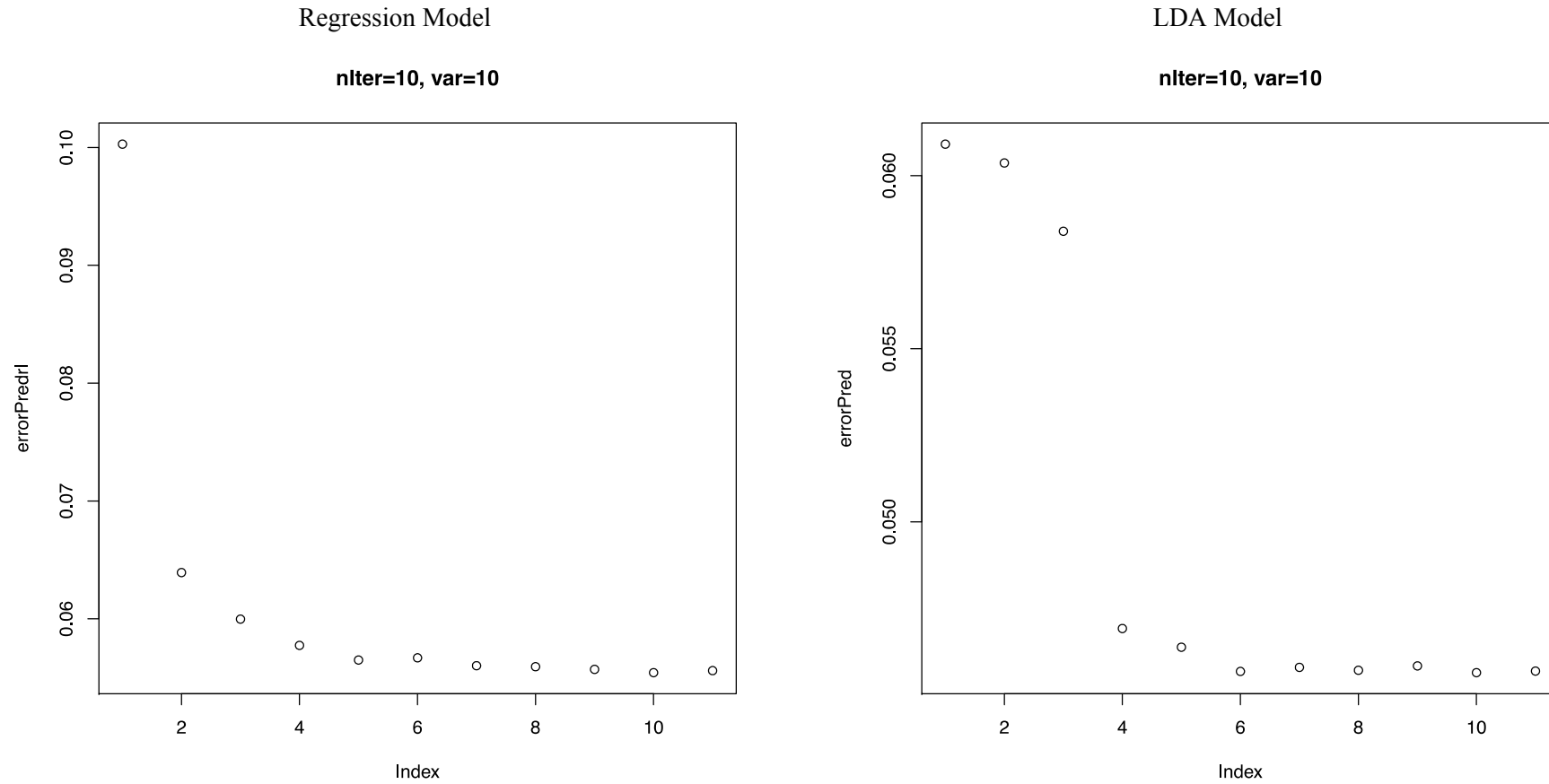
Figure 5. Forward stepwise for classification problems with GEM 2014 Individual Level data
