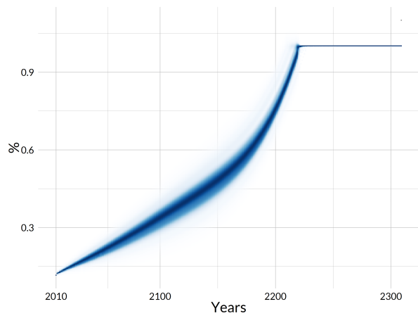
(b) Abatement rate
