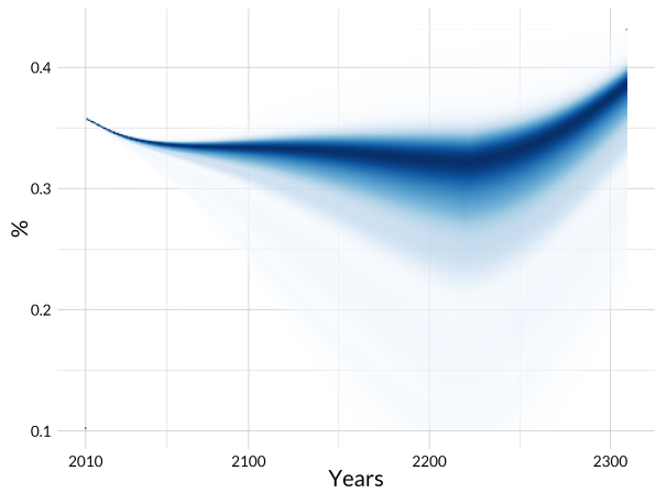
(c) Investment rate
