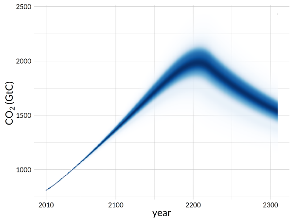
(a) CO_2 level
