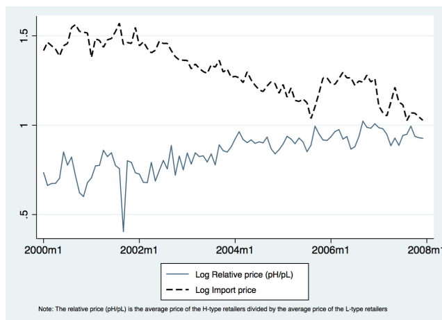
Figure 3: Import price and relative price of H- and L-type retailers
