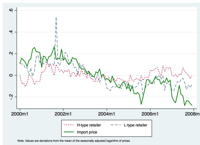
Figure 2: Import price and average price for H- and L-type retailers
