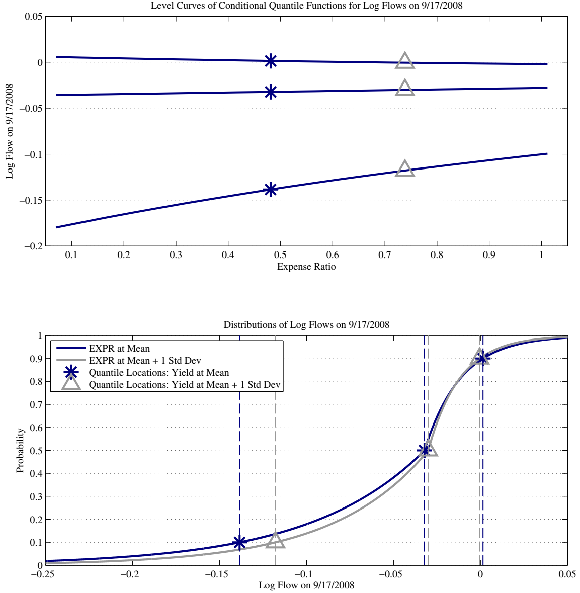
Figure 4: Marginal Effects of Expense Ratio on Log Flow Distribution for 9/17/2008 - Prime Institutional Funds
