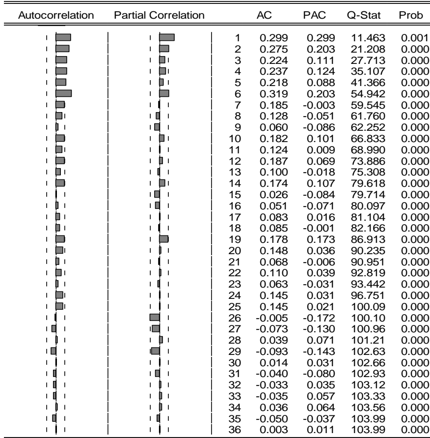
Fig 3: ACF and PACF Plot of \text{dlog}(ER_t)
