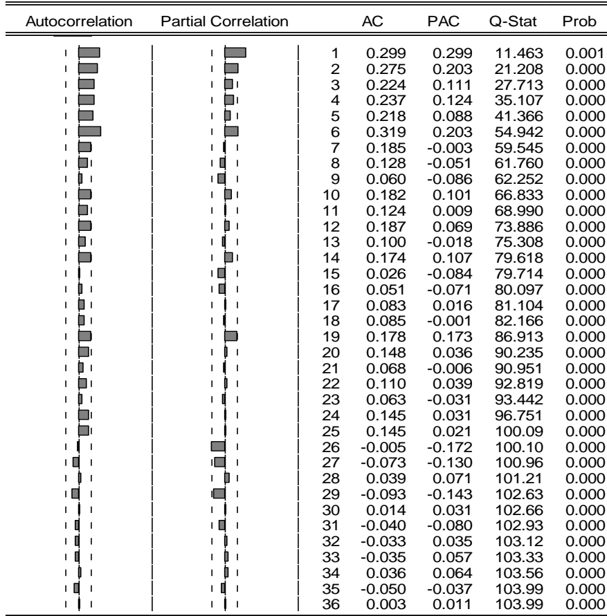
Fig 3: ACF and PACF Plot of \text{dlog}(\text{ER}_t)
