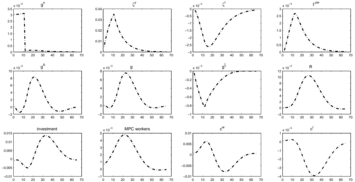
Figure 4: Simulation: baby-boomers
