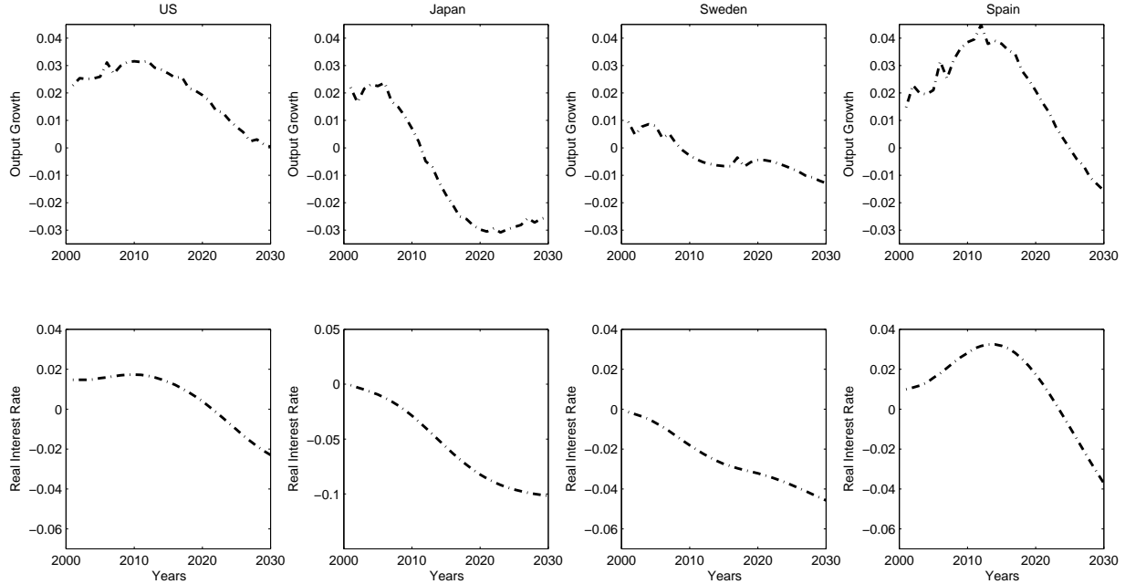
Figure 6: Simulation: prediction
