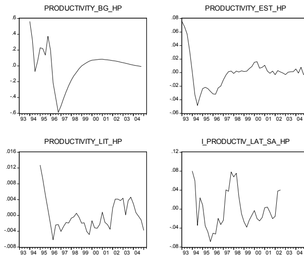
Fig.2 Productivity fluctuations, 1993-2005
