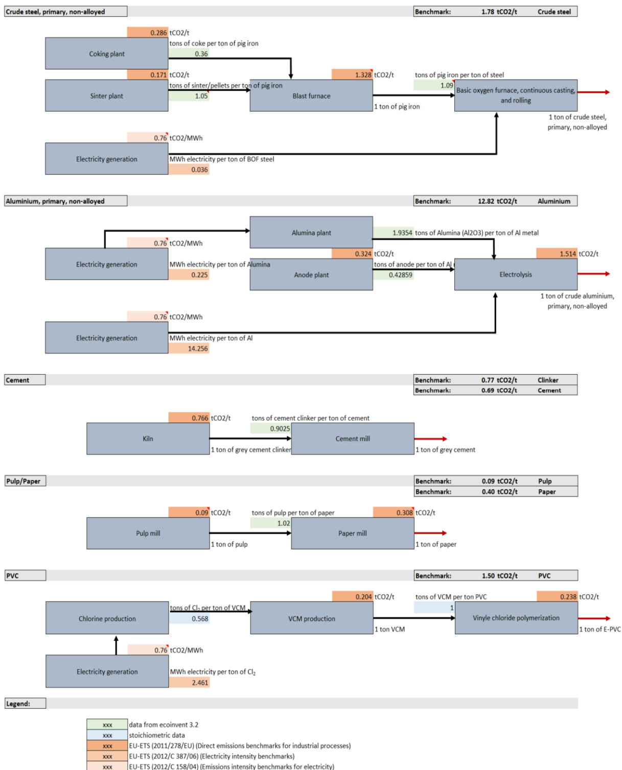
Figure A1. System definition for the derivation of product-specific emissions benchmarks for the five materials studied. The process chains were built using data from ecoinvent (Ecoinvent Centre, 2014) and stoichiometric information. The EU-ETS emissions benchmarks for processes define the scope of the process chains and the emissions multipliers.
