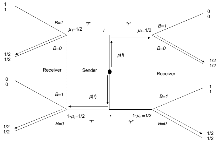
Figure 1. Rendez-vous : Uninformative Equilibrium where Message are Disregarded
