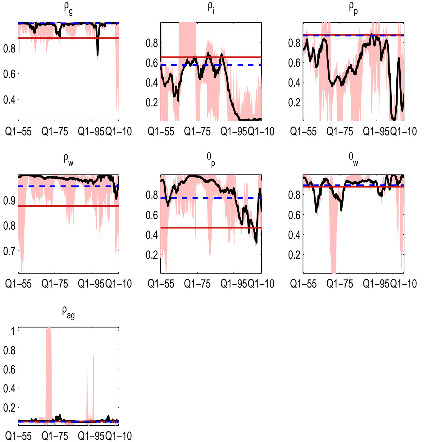
Figure 7: Time-varying DSGE parameters: IV
