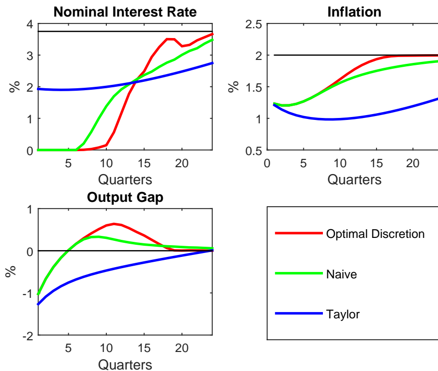
Figure 2: Liftoff in the backward-looking model
