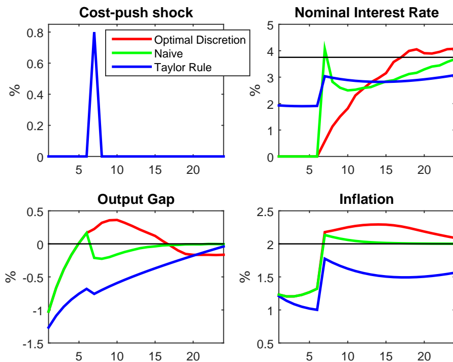
Figure 3: Large cost-push shock in the backward-looking model
