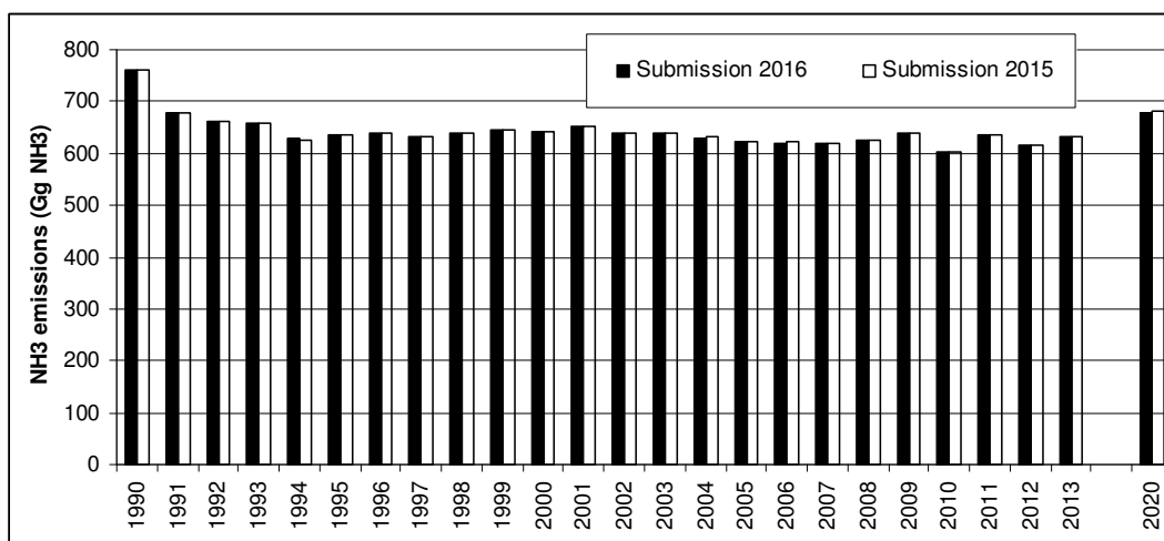
Figure 2.14: Comparison of NH 3 emission results in Submission 2016 and Submission 2015
