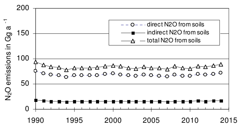
Figure 2.5: N_2O emissions from agricultural soils (in Gg a^{-1} N_2O ), Submission 2016
