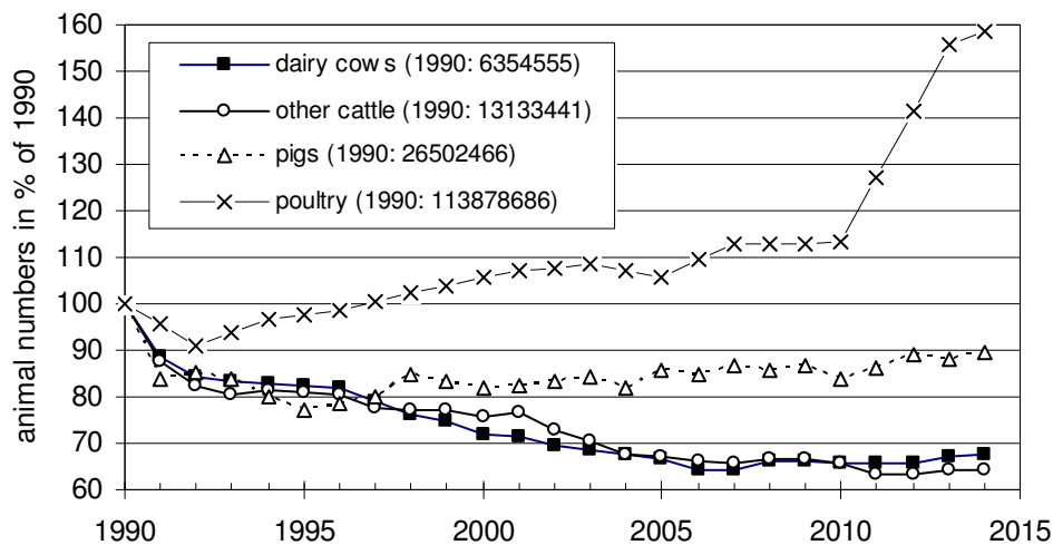
Figure 2.3: Development of animal numbers in % of 1990, Submission 2016
