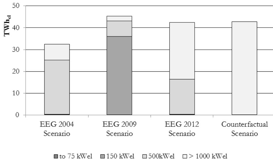
Figure 3: Electricity production under different scenario settings
