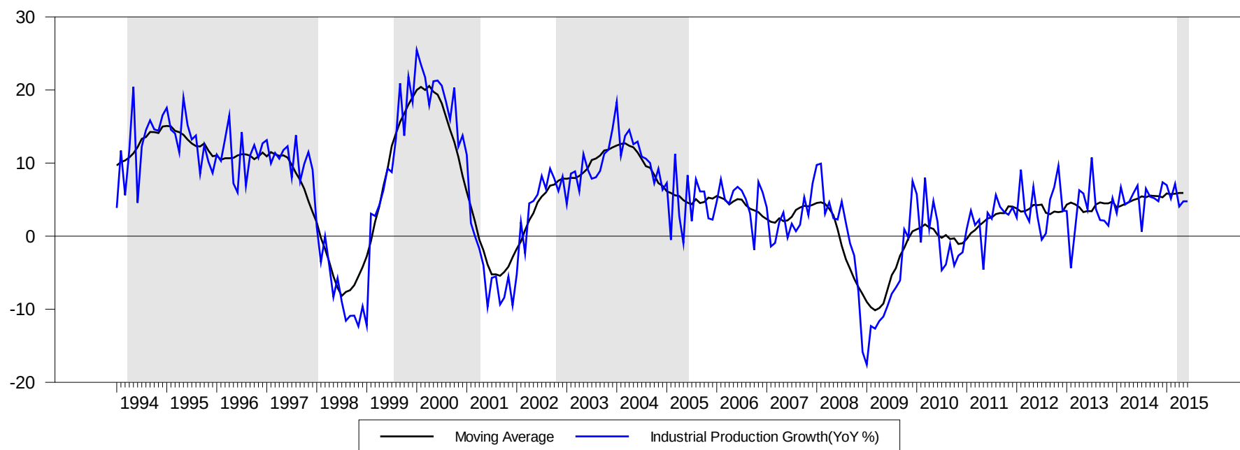
Figure 1. Regime classifications.
