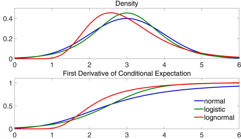
Figure 2: Predicted matching coefficients for standard distributions
