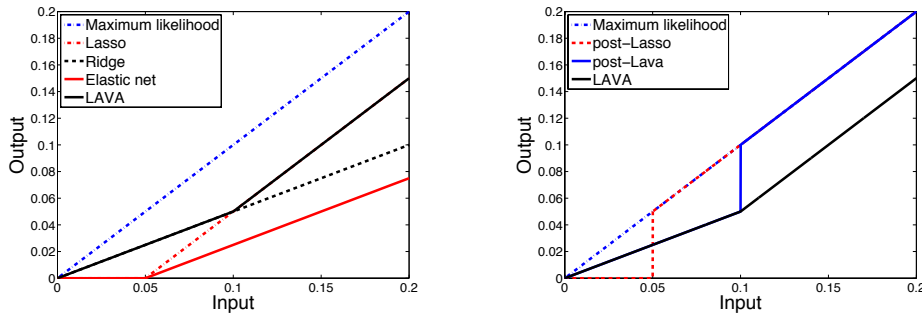
FIG 2. Shrinkage functions. Here we plot shrinkage functions implied by lava and various commonly used penalized estimators. These shrinkage functions correspond to the case where penalty parameters are set as \lambda_2 = \lambda_r = 1/2 and \lambda_1 = \lambda_l = 1/2 . In each figure, the light blue dashed line provides the 45 degree line coinciding to no shrinkage.
