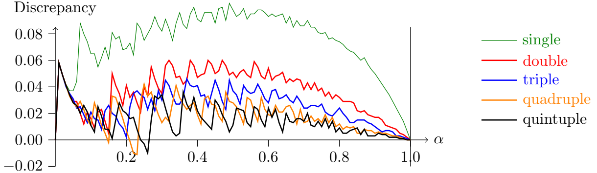
Figure 4: n = 100, \theta = -0.99
