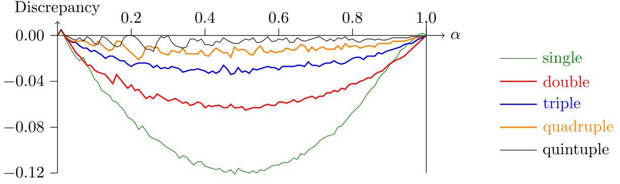
Figure 2: n = 100, \theta = -0.90
