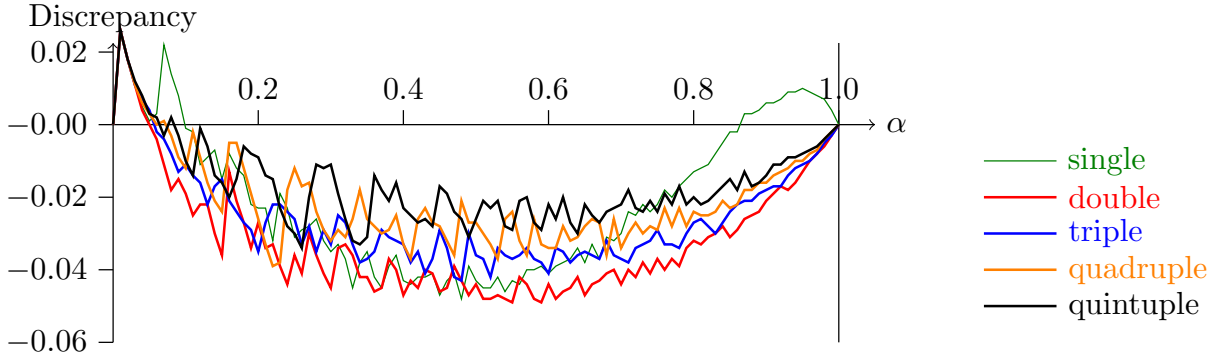
Figure 3: n = 100, \theta = -0.95
