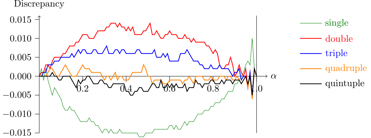
Figure 5: n = 100 , \theta = -0.70
