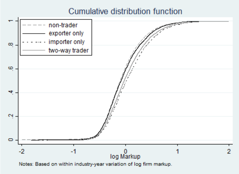
Figure 1: Cumulative distribution function of markups by trading status
