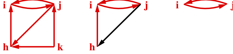
Figure 2: From left to right: Graph representation of the original opinion profile and the profiles of the restricted games which correspond to the first and second iteration of the eliminative TC-algorithm. Red arcs indicate top candidate relation.
