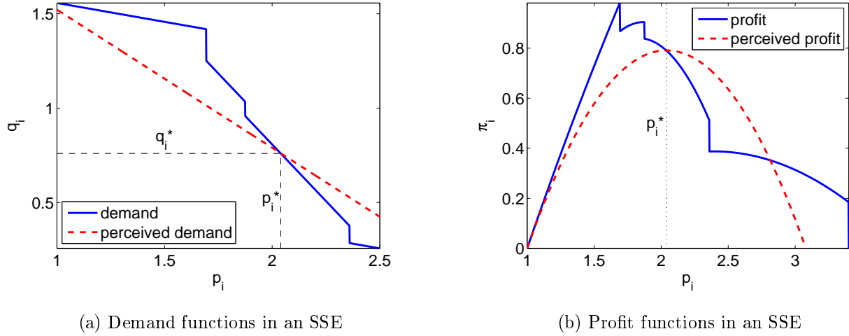
Figure 2: Demand and profit functions of firm i in a self-sustaining equilibrium. Parameters: s = 1 , S = 5 and c = 1 . Equilibrium prices: p_i^* = 2.0398 , p_j^* = 2.0264 and p_k^* = 2.2083 .
