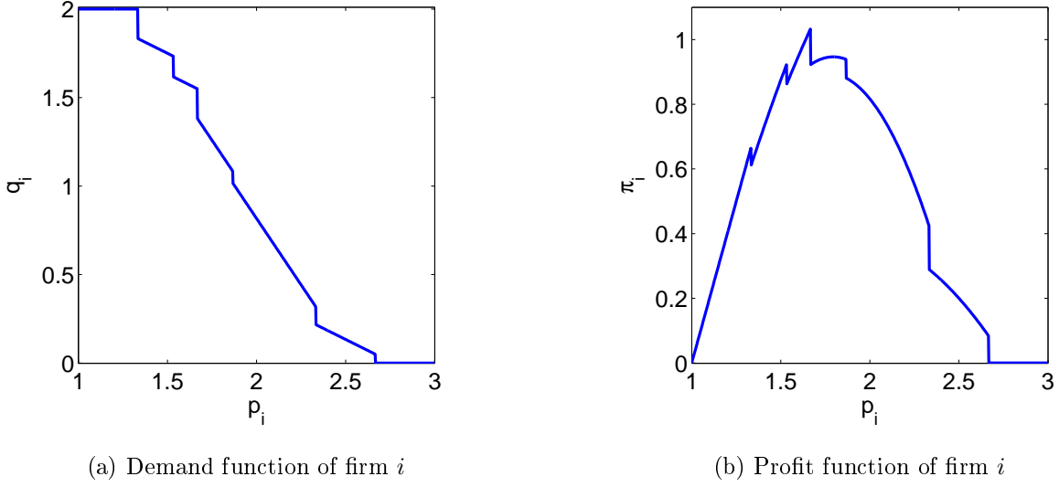
Figure 1: Demand function of firm i for p_j = 2 and p_k = 2.2 . Other parameters: s = 1 , S = 2 and c = 1 .
