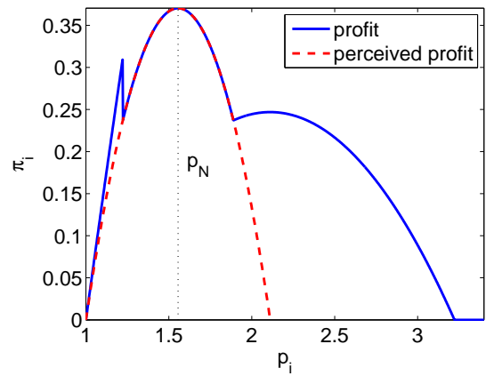
(b) Profit functions (Nash equilibrium)
