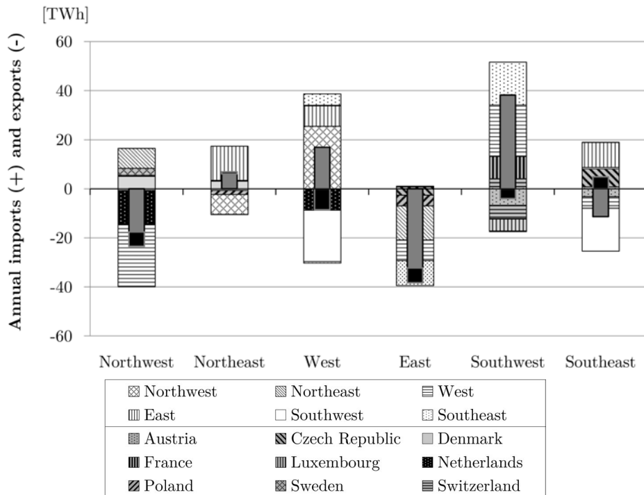
Figure 16: Annual electricity exchange with neighboring zones and countries
