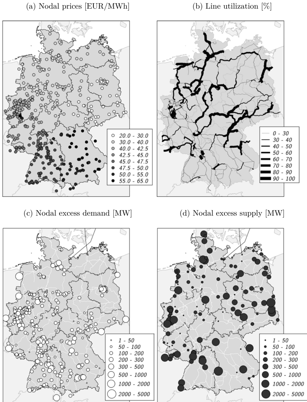
Figure 7: High winter demand, no PV, and very high wind generation (h2)
