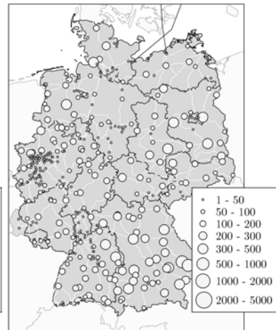
Figure 4: Renewable capacities of conventional power plants [MW]
