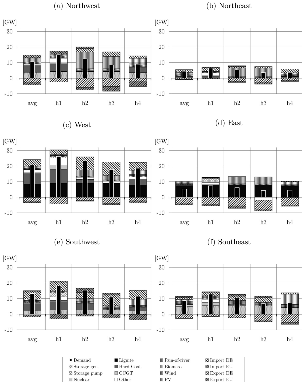
Figure 11: Zonal generation, demand, and trade for exemplary hours (h1–h4)
