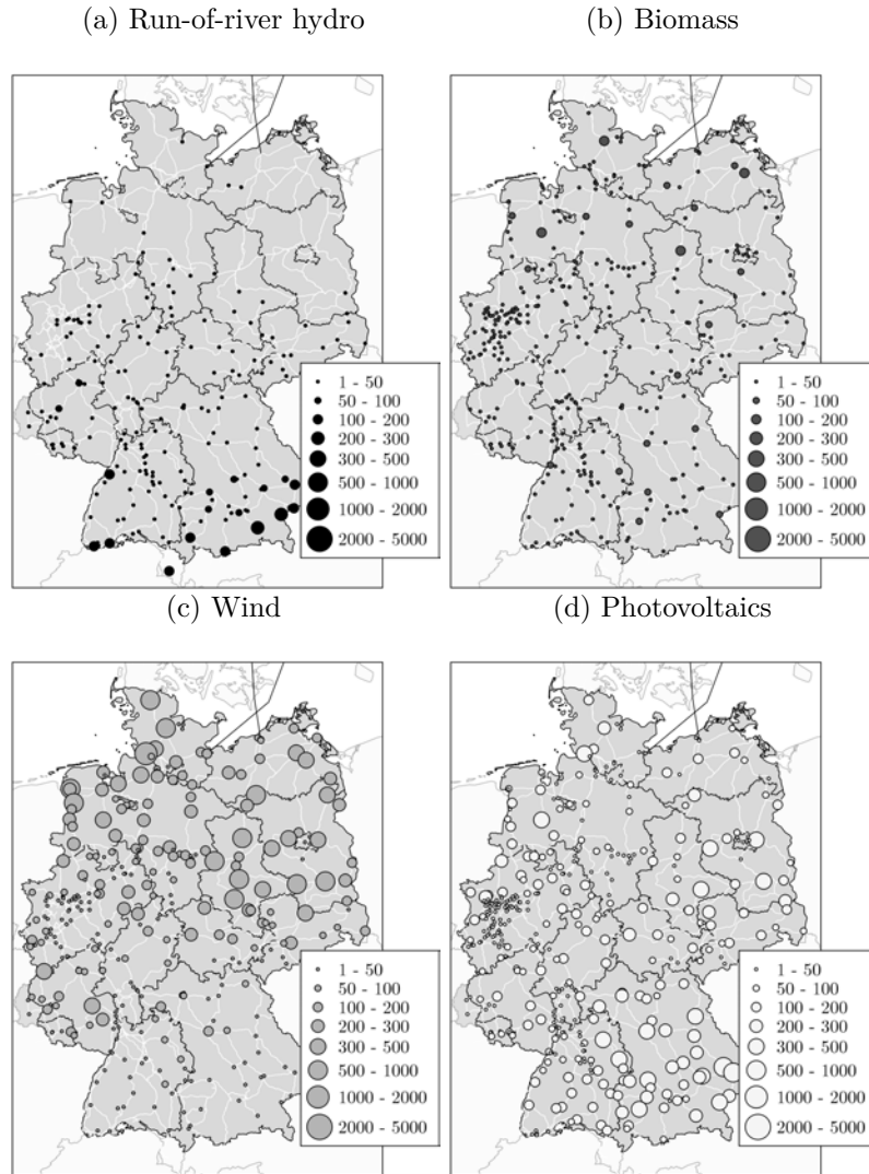
Figure 4: Renewable capacities of conventional power plants [MW]
