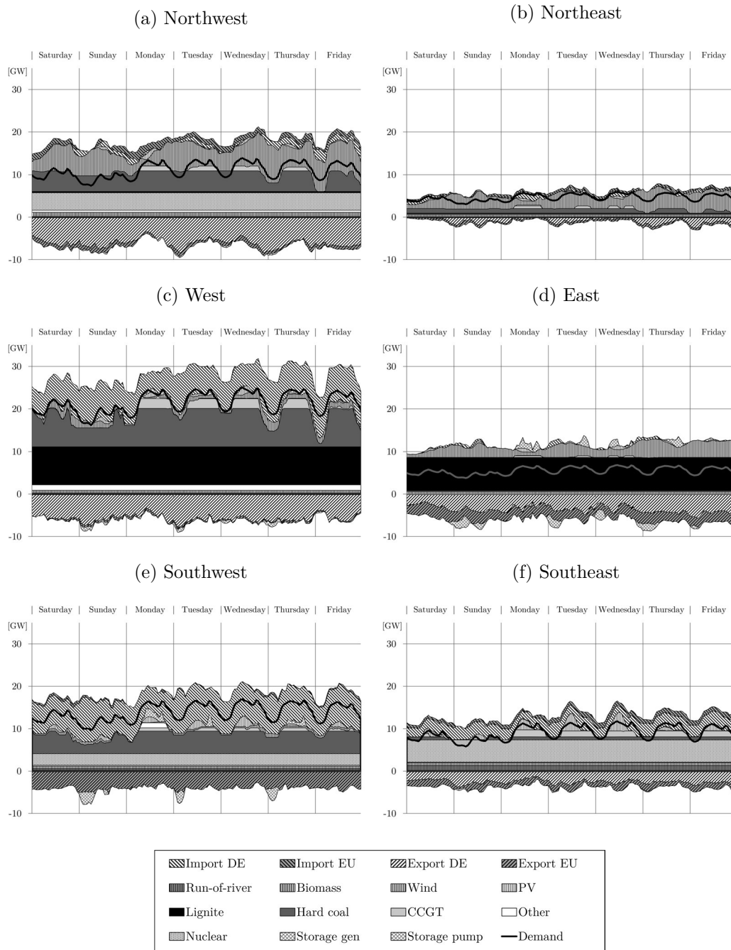
Figure 13: Zonal generation, demand, and trade for one winter week
