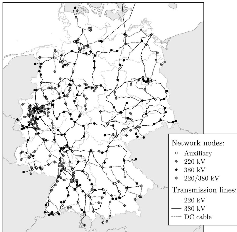
Figure 2: High-voltage transmission network in 2012
