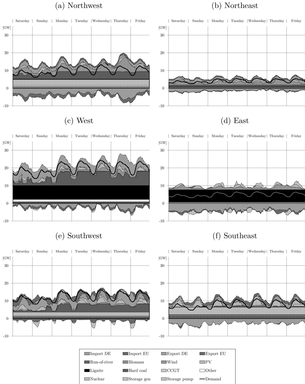
Figure 15: Zonal generation, demand, and trade for one summer week
