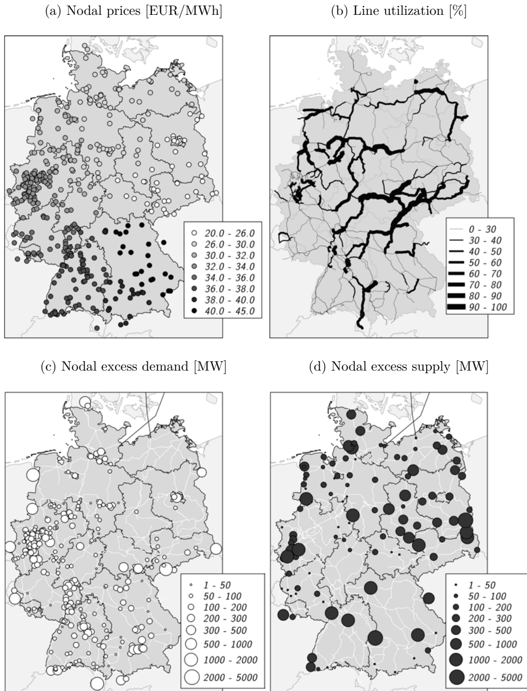
Figure 8: Low winter demand, no PV, and high wind generation (h3)
