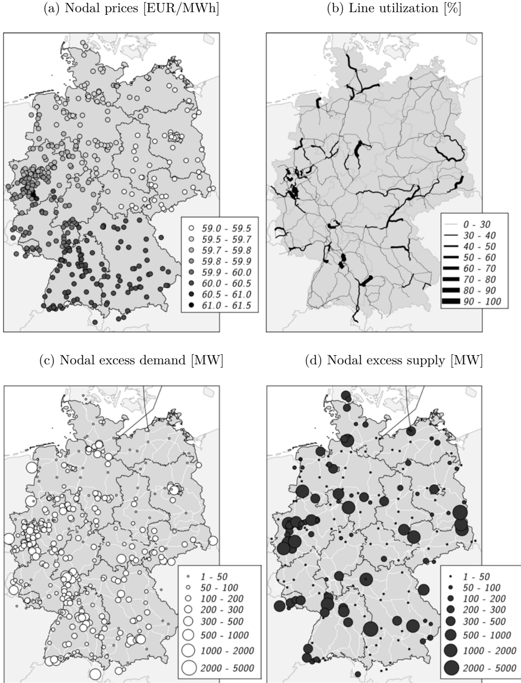
Figure 5: Average for all hours of nodal model results (avg)
