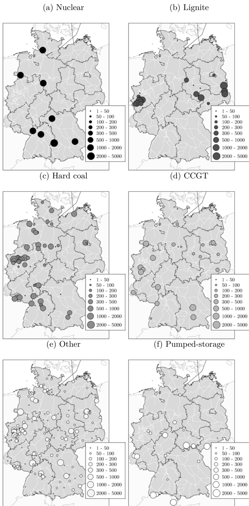
Figure 3: Generation capacities of conventional power plants [MW]
