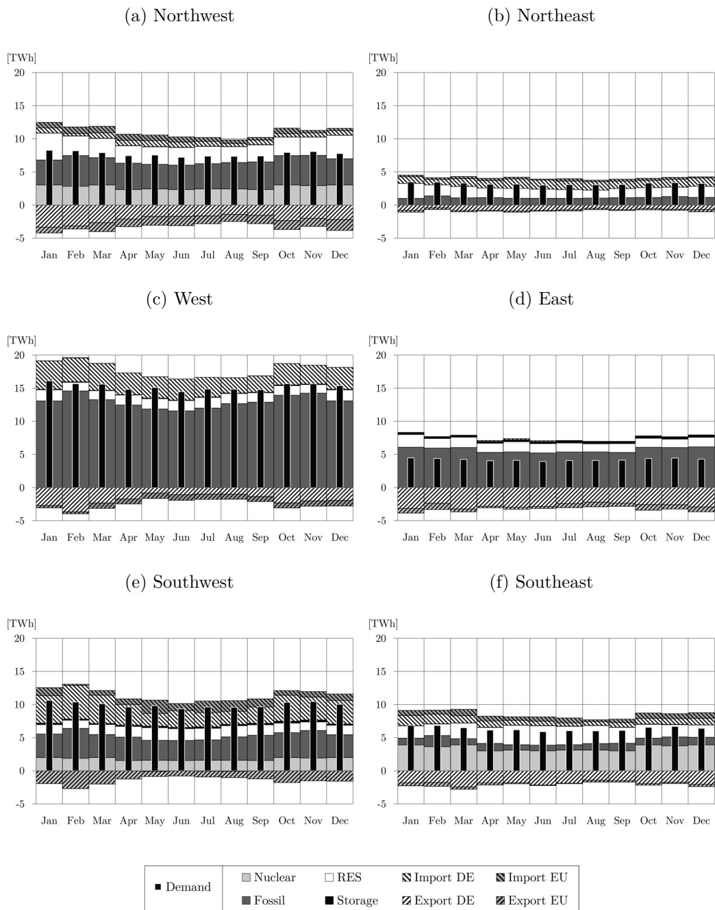
Figure 17: Zonal generation, demand, and trade levels by month for six zones
