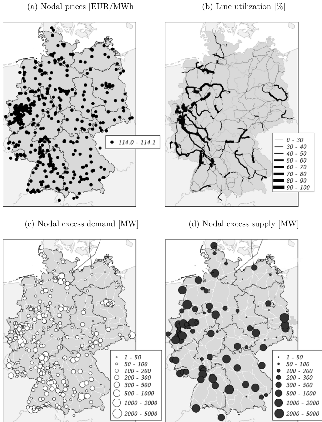
Figure 6: Peak winter demand and low renewable generation (h1)
