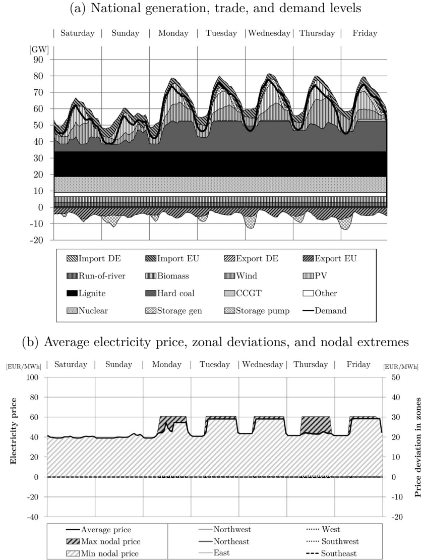
Figure 14: Hourly system state and electricity prices of one summer week
