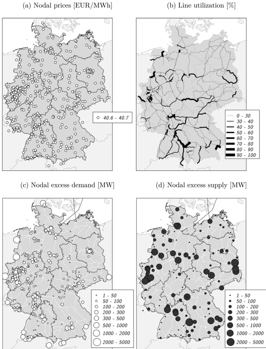
Figure 9: Low summer demand, high PV, and low wind generation (h4)
