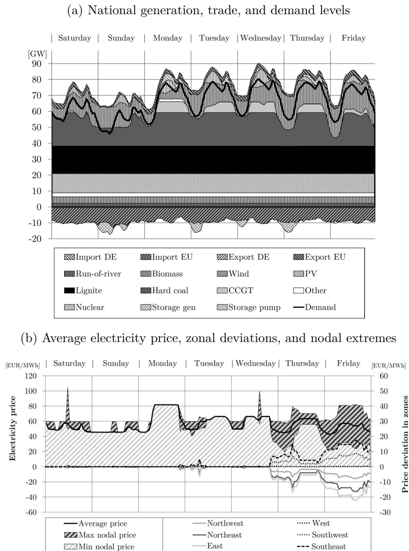
Figure 12: Hourly national results and electricity prices for one winter week
